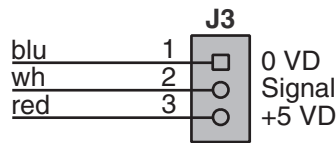
Figure 4. J3 60-bit Speed Connector
